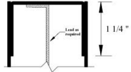
Top & Bottom Channel 16 ga A-60
